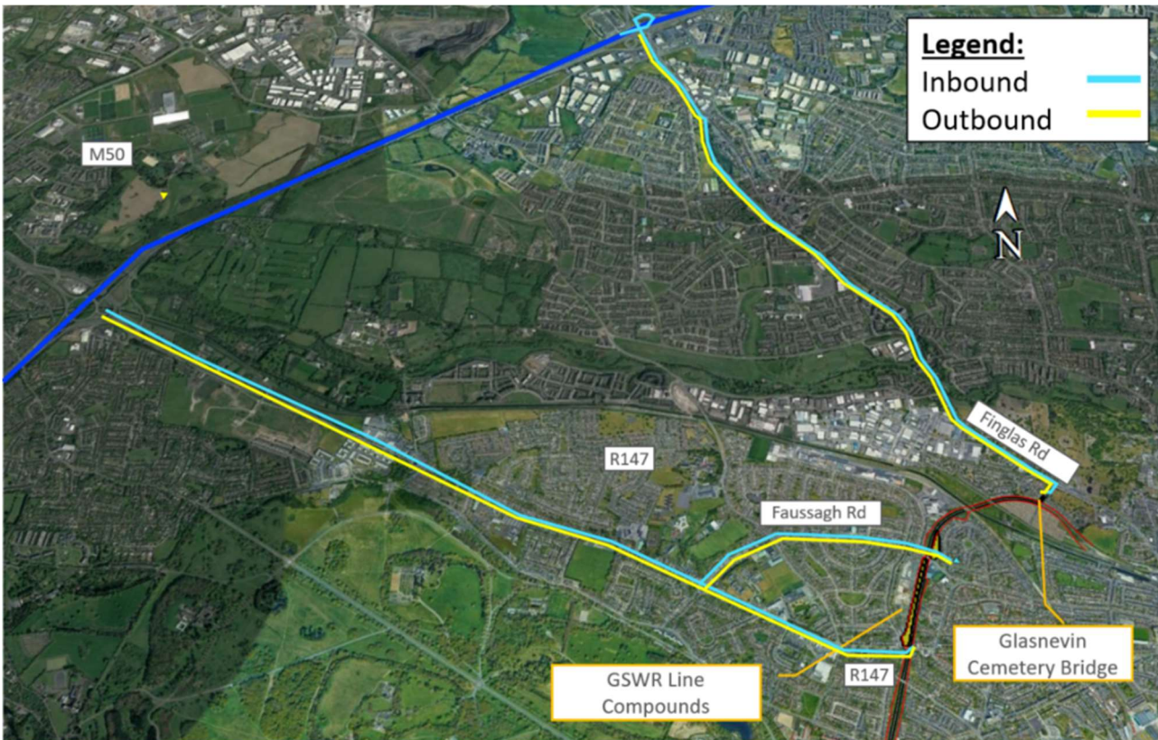
Figure 5-136 Zones D-2 & D-3: PPTBL & Glasnevin Cemetery Bridge Compound Haul Routes
