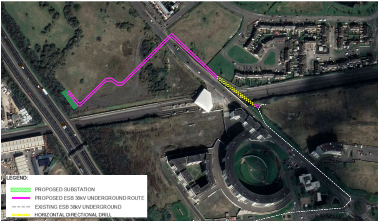
Figure 5-32 Park West Substation Proposed Grid Connection
