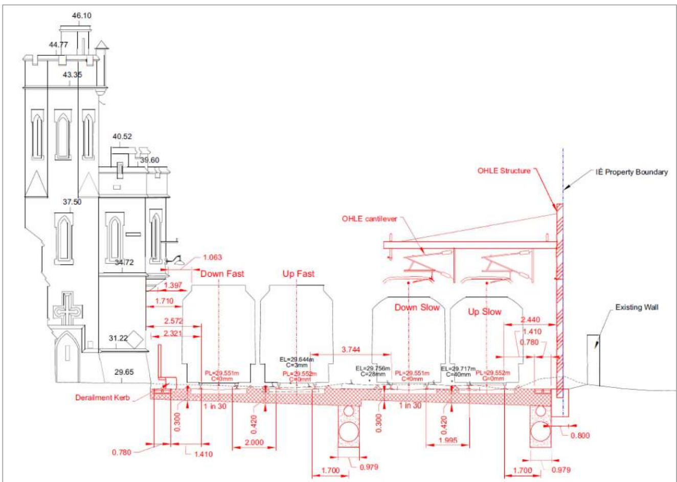
Figure 5-66 Cross Section at Ch 11+000 - Inchicore - Facing West
