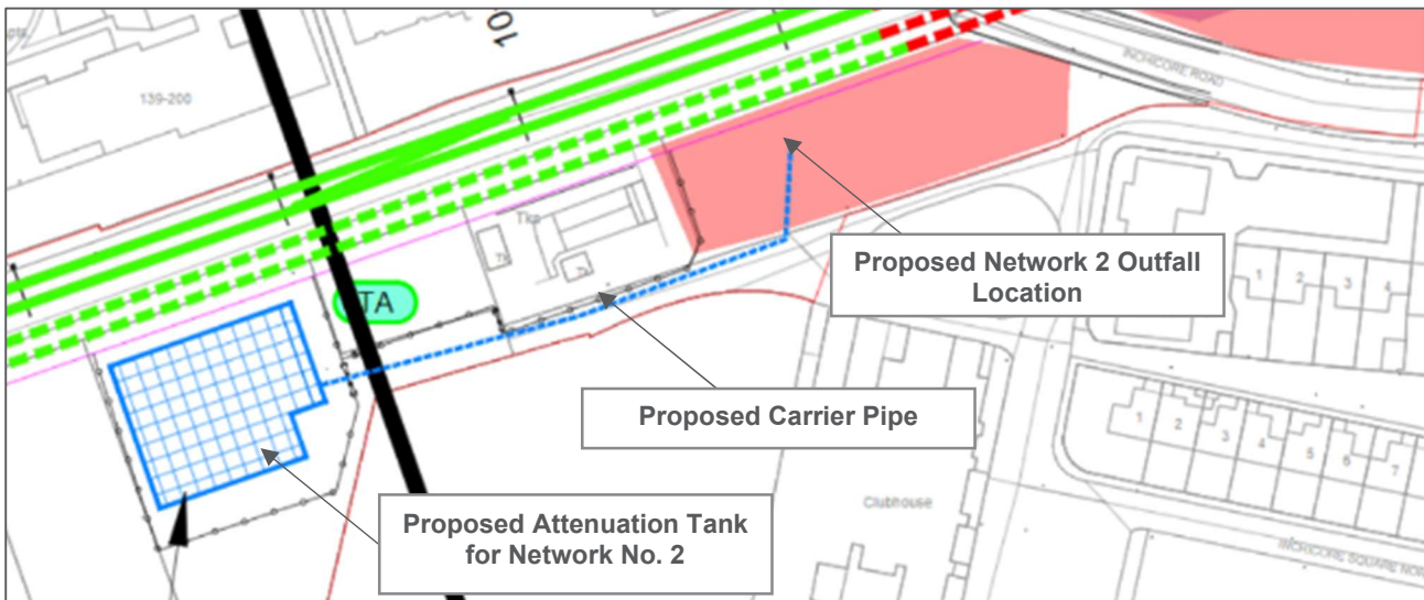
Figure 5-76 Network 2 Attenuation Tank Layout
